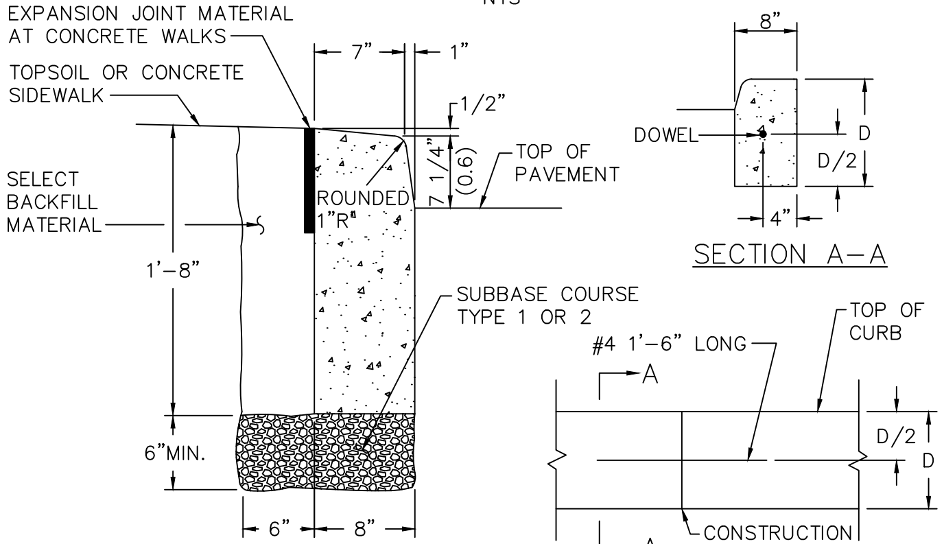
CURB AT FLEXIBLE PAVEMENT
